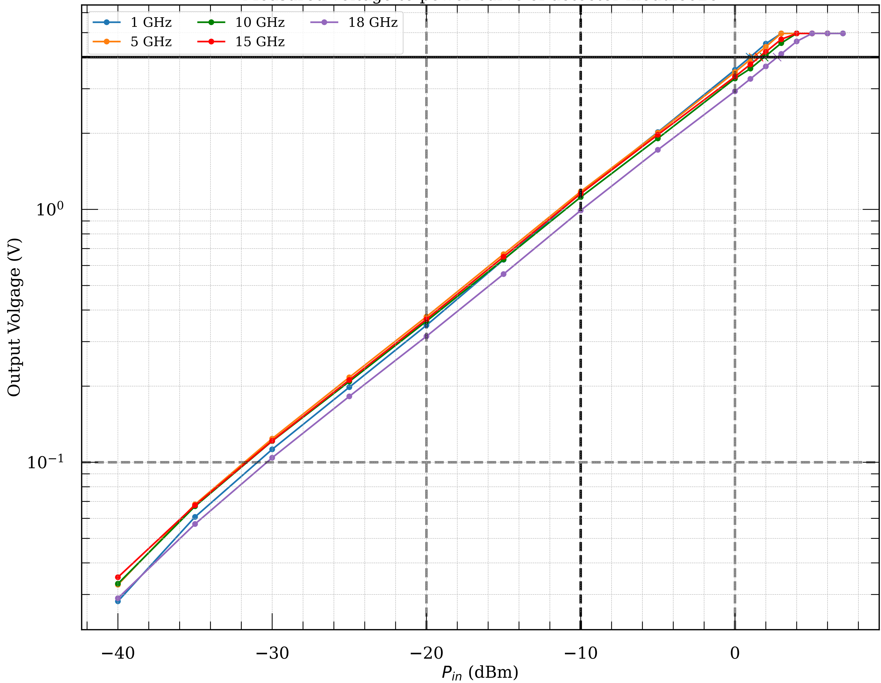
Measured voltage-to-power curve of detector module026
